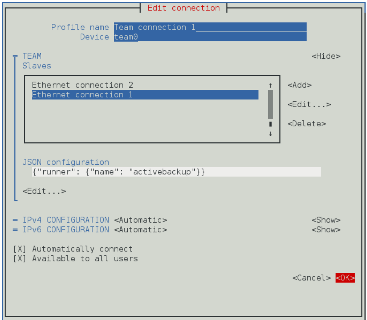
Figure 5.5. The NetworkManager Text User Interface Configuring a Team Connection menu
