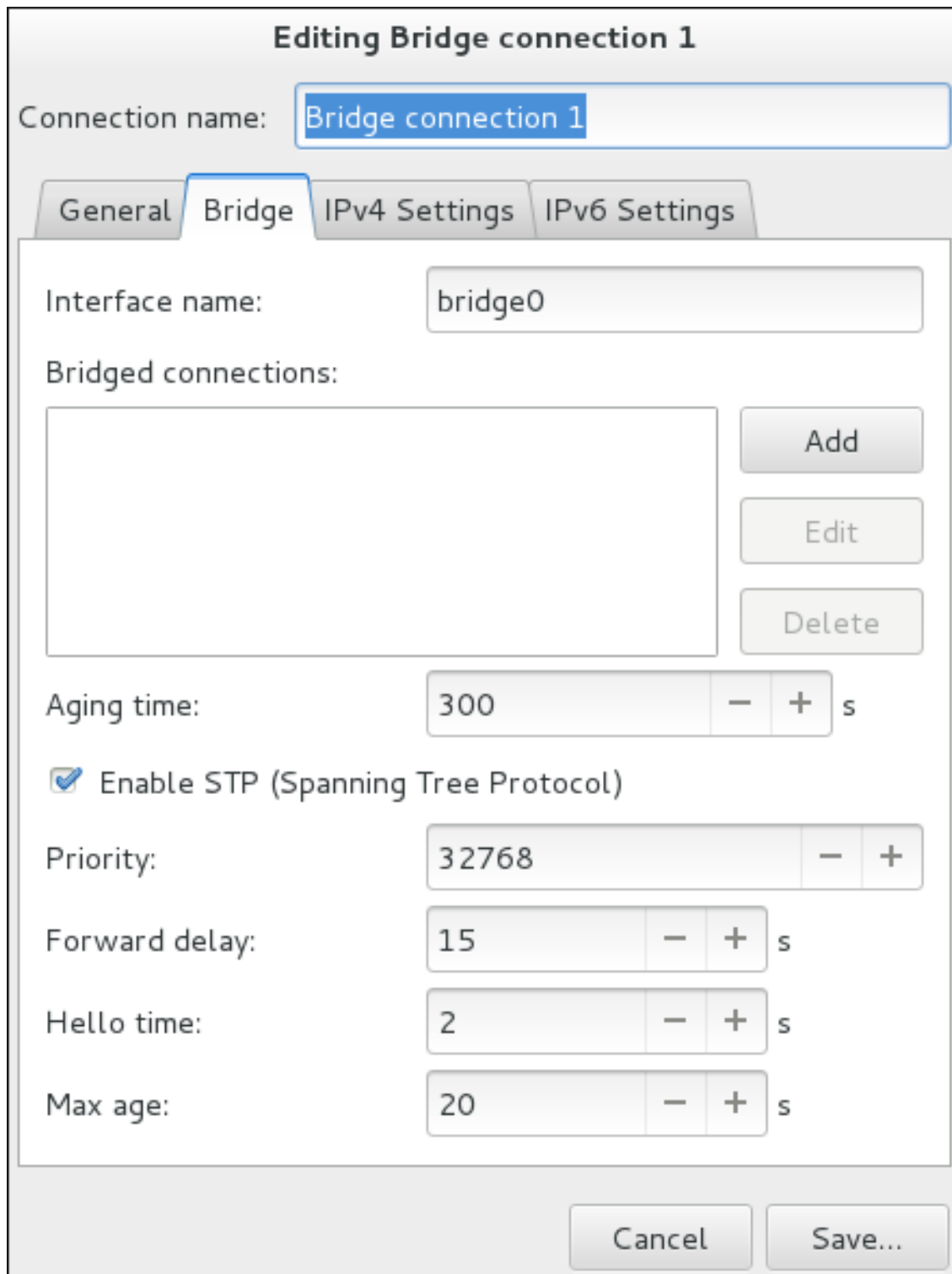
Figure 6.5. Editing Bridge Connection 1
