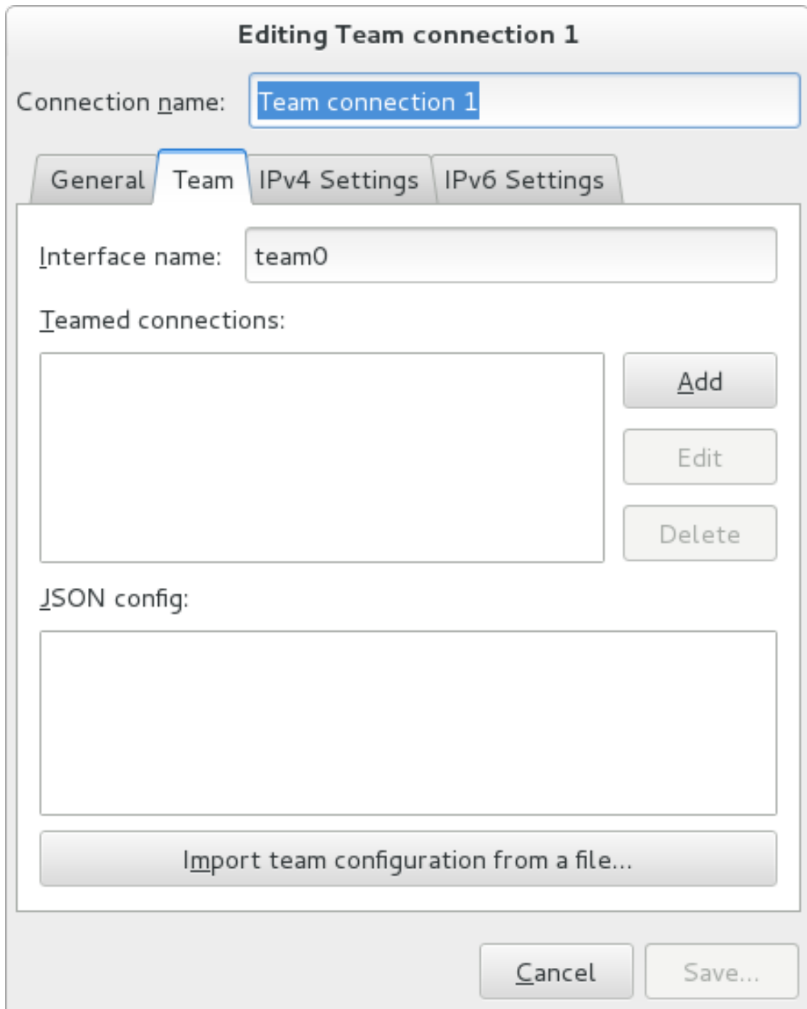
Figure 5.6. The NetworkManager Graphical User Interface Add a menu
