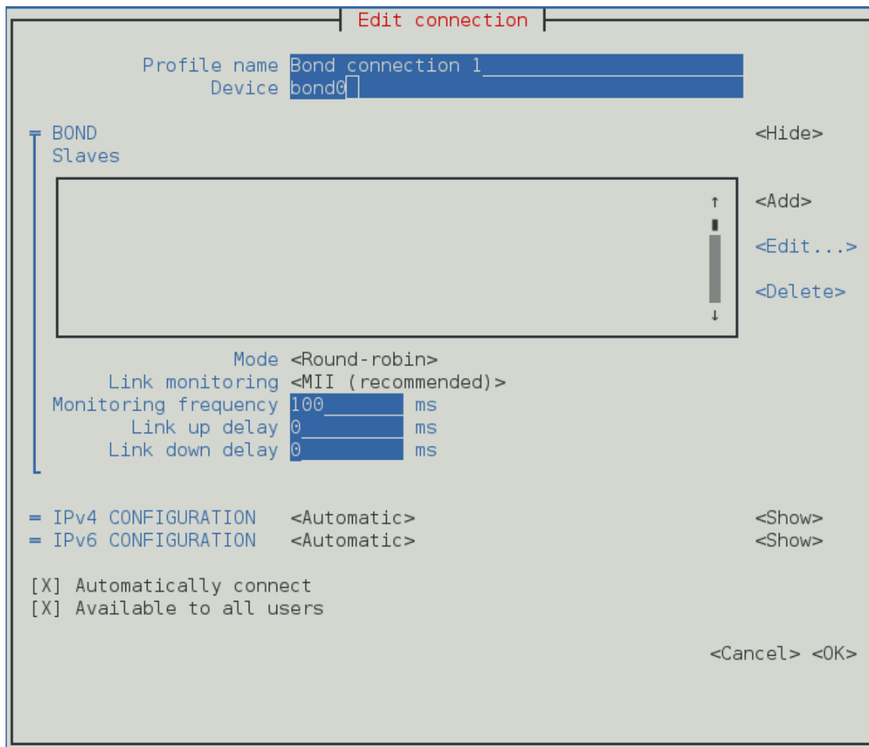
Figure 4.2. The NetworkManager Text User Interface Configuring a Bond Connection menu
