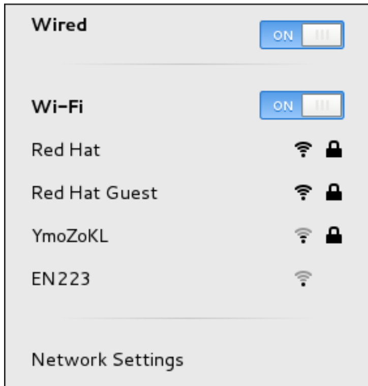
Figure 2.3. The GNOME network menu, showing all available and connected-to networks
