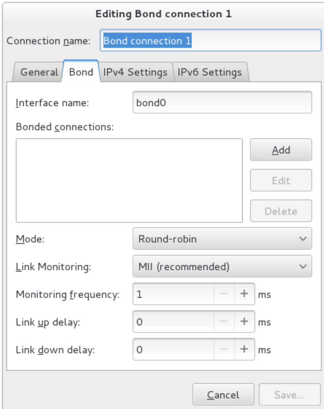
Figure 4.6. The NetworkManager Graphical User Interface Add a Bond menu
